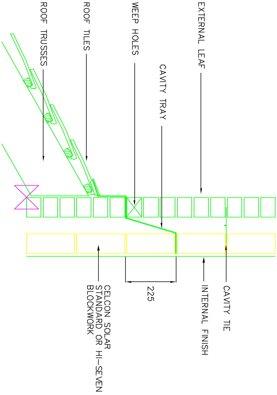
SECTION THROUGH CAVITY WALL AT LEAN TO ROOF ABUTMENT
