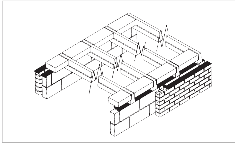
Figure 1 Typical floor arrangement
